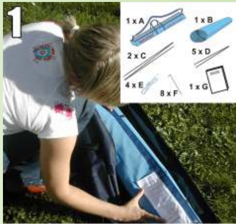
Remove the HelioTent from the carrying bag. Note: Some parts are located in the side pocket of the carrying bay. Poles „C“ will be visible after unrolling HelioTent at step 4.
